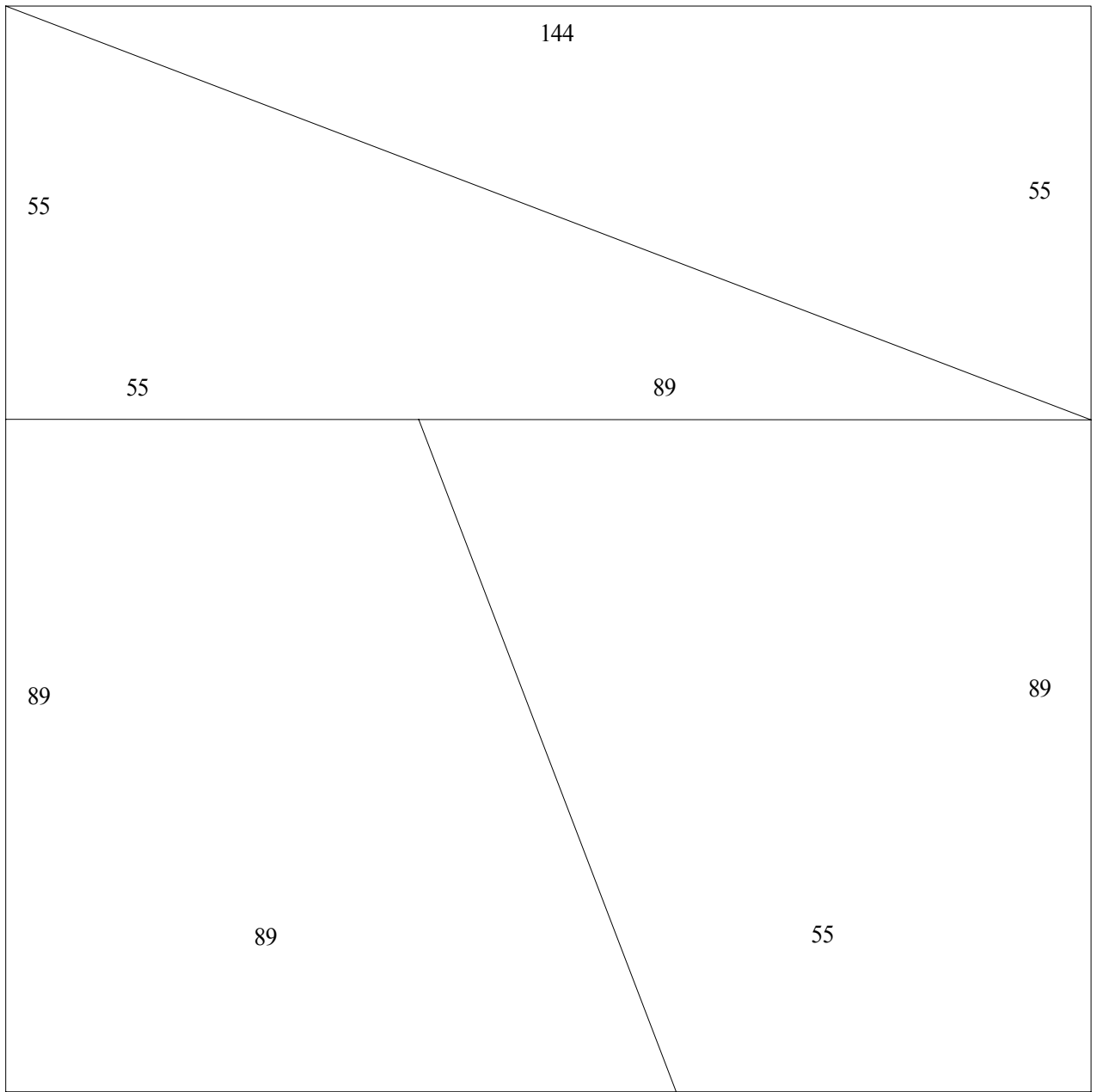
"Fibonacci" Division of a Square
