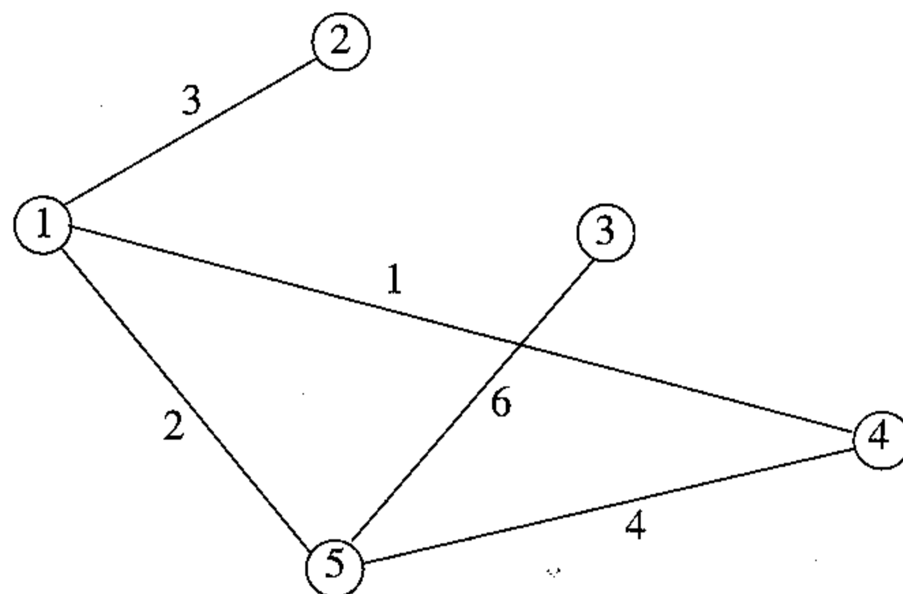
Figure 4.1. A connected graph with arc weights.
