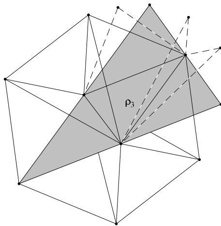
Figure 4: The tessellation \{3, \infty\} cutting through \{3, 3, 6\} .
