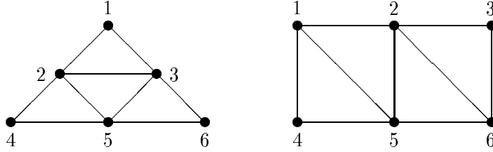
FIGURE 1. The graphs \Gamma and \Gamma'
