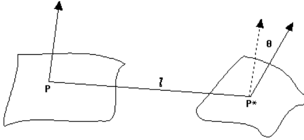
Figure 3: Pseudospherical line congruence
